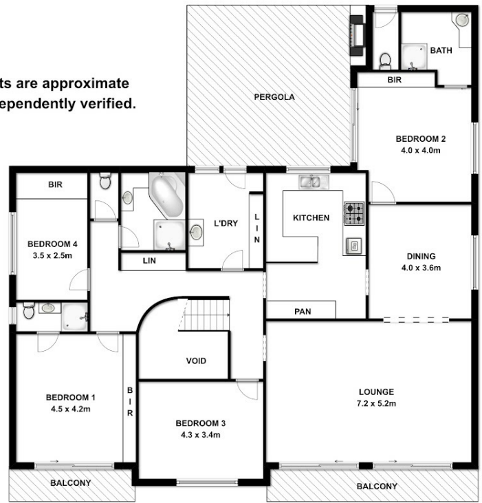
UPPER FLOOR
