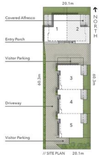
// SITE PLAN 20.1m 60.3m BLAKE STREET
