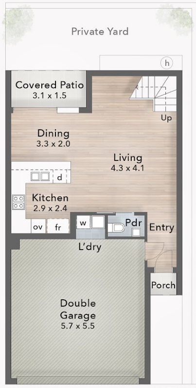
// FLOOR PLAN Ground Floor - Townhouse 4 2.7m Ceiling
