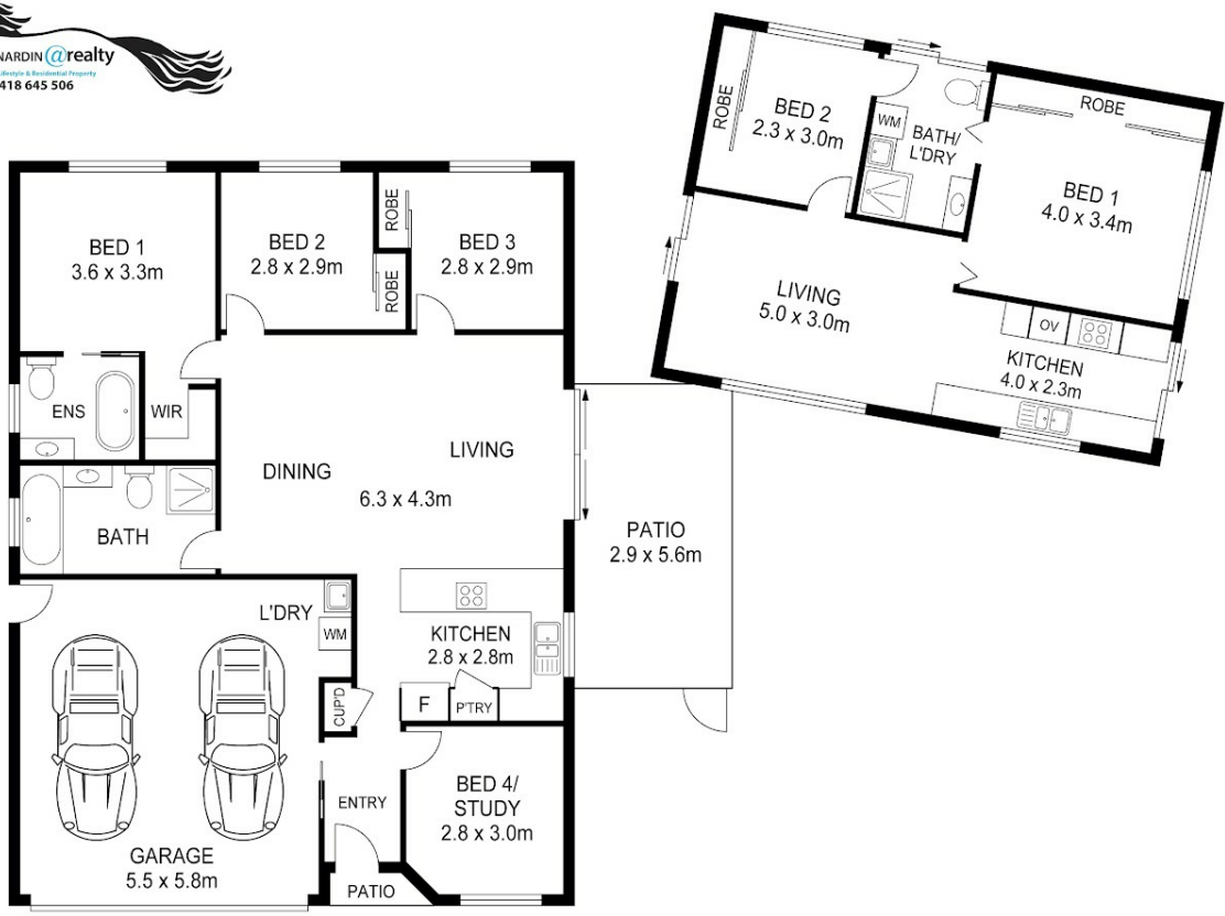
0m 1m 2m 3m 4m 5m SCALE (METRES) PLANS SHOWN ONLY INDICATIVE OF LAYOUT. DIMENSIONS ARE APPROXIMATE.
