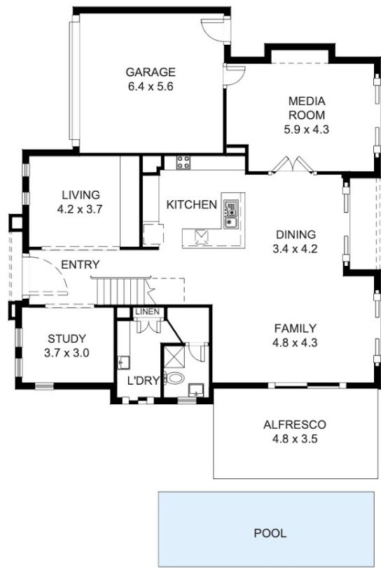
GROUND PLAN
