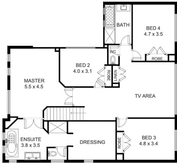
FIRST PLAN
