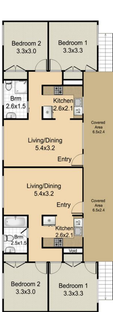
UPPER FLOOR
