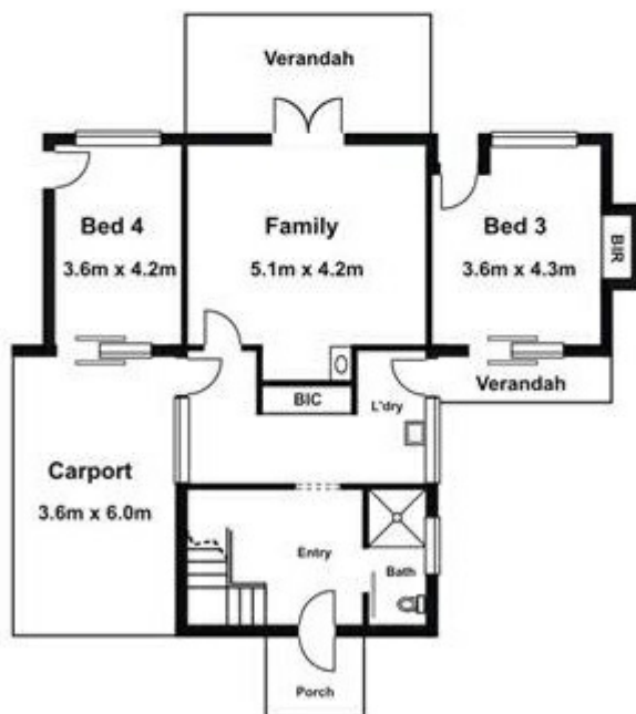
Lower Floor
