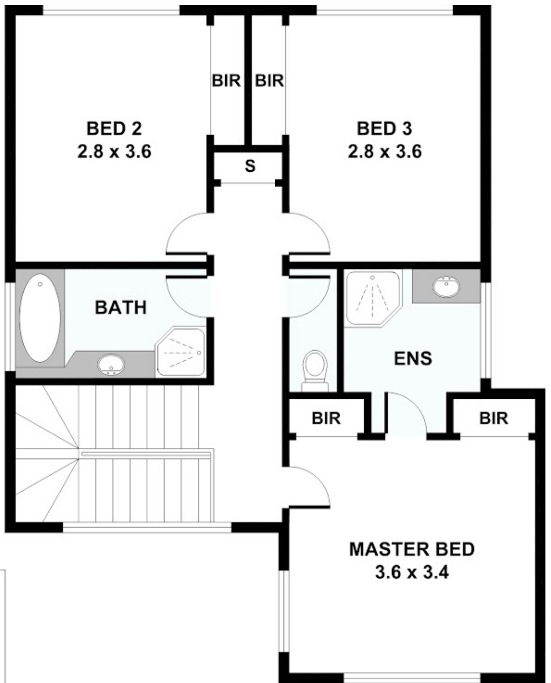
FIRST FLOOR
