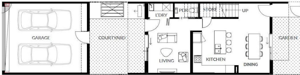
GROUND FLOOR
