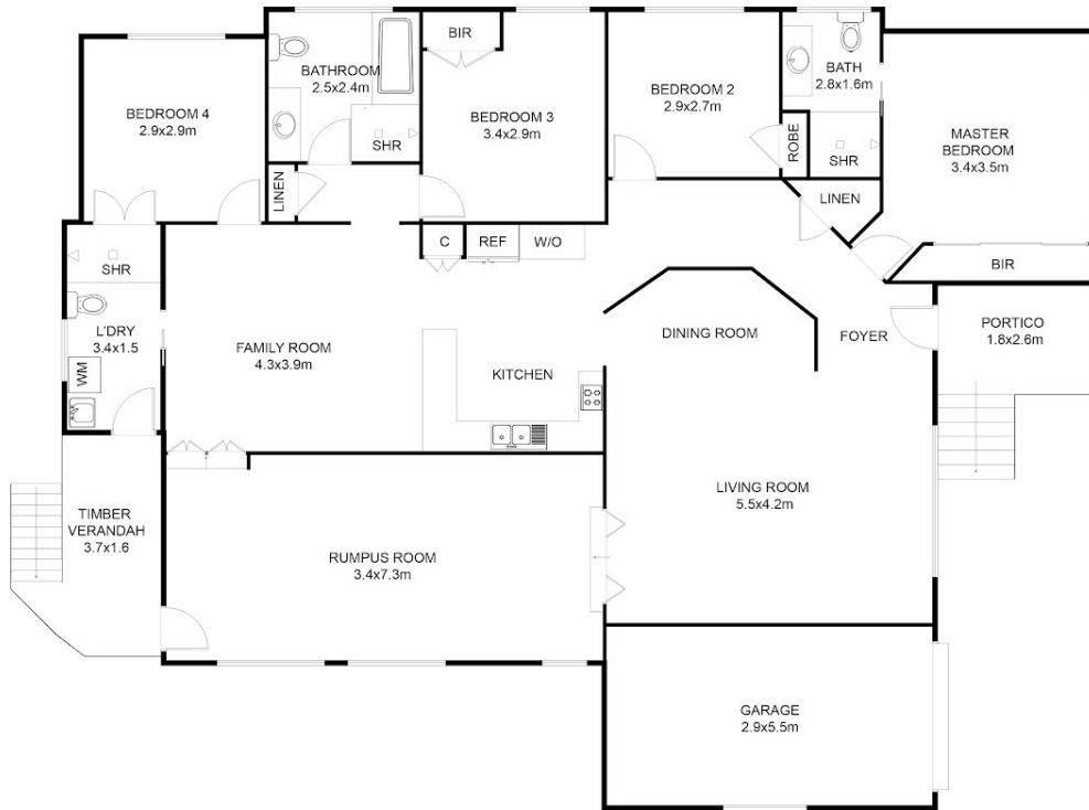
FLOOR PLAN
