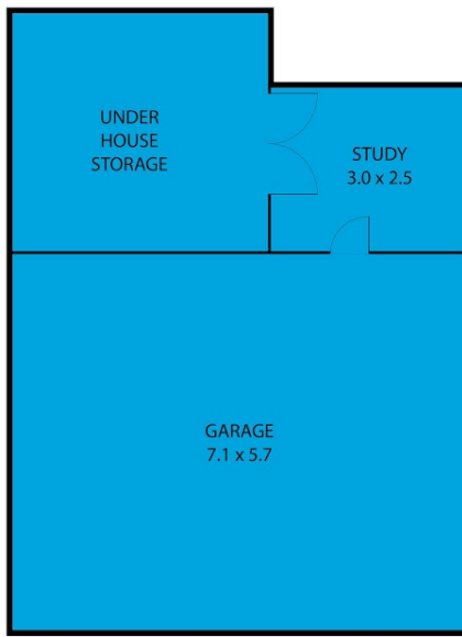
LOWER LEVEL
