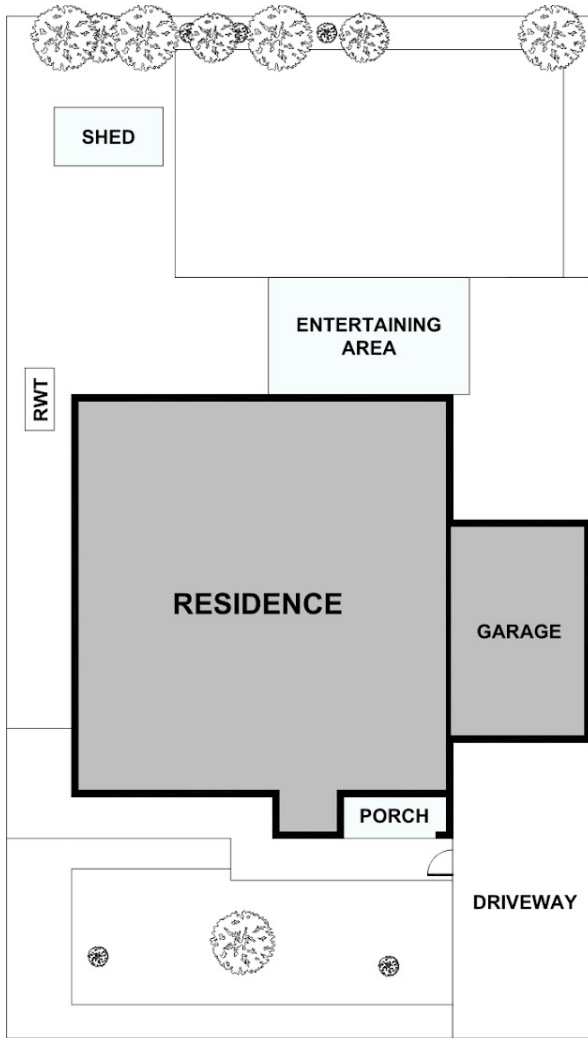
SITE PLAN
