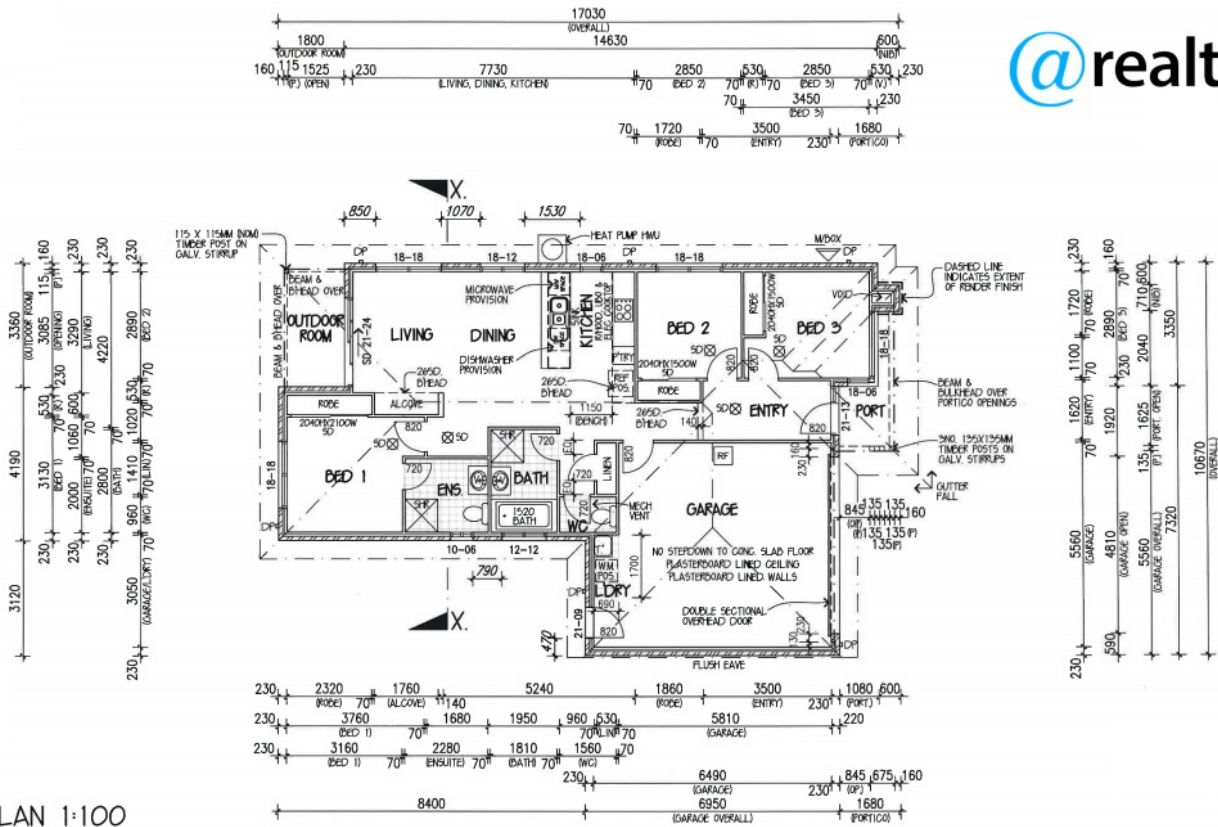
FLOOR PLAN 1:100
