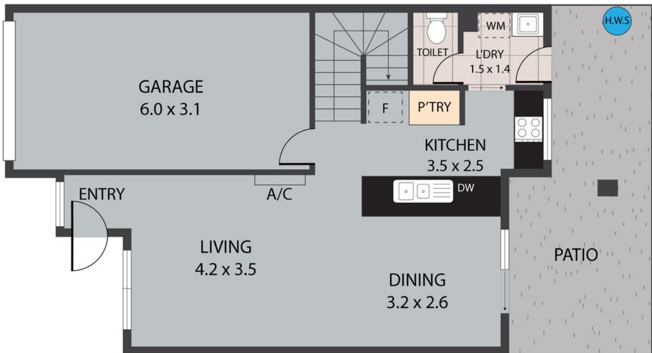
GROUND FLOOR
