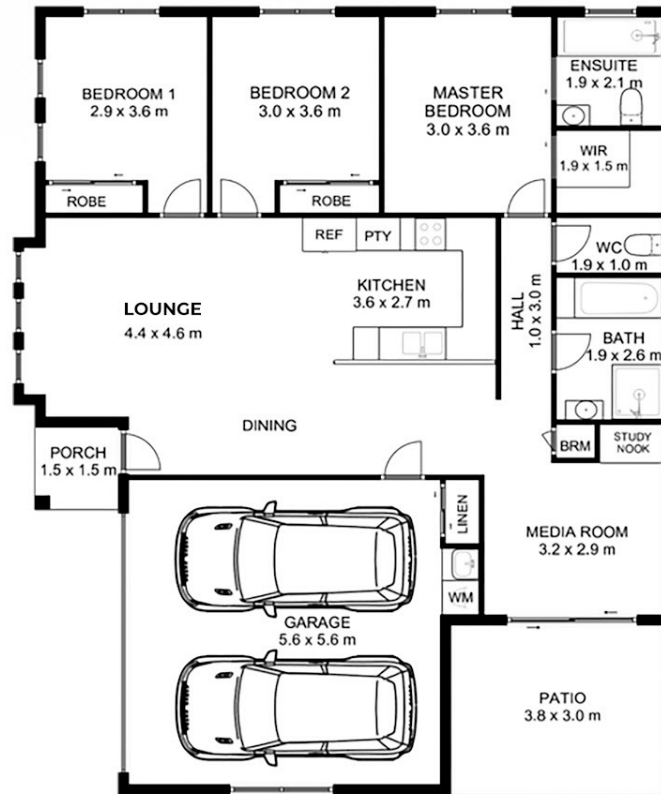
GROUND LEVEL
