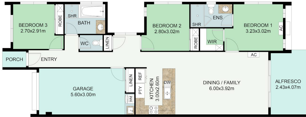
FLOOR PLAN
