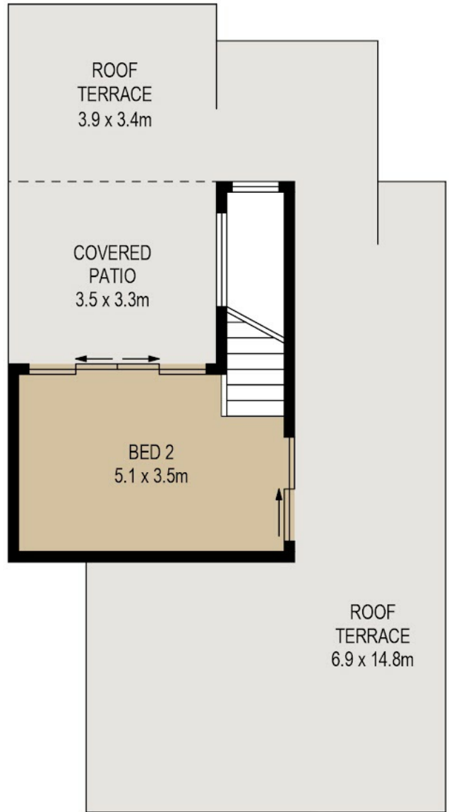
UPPER LEVEL
