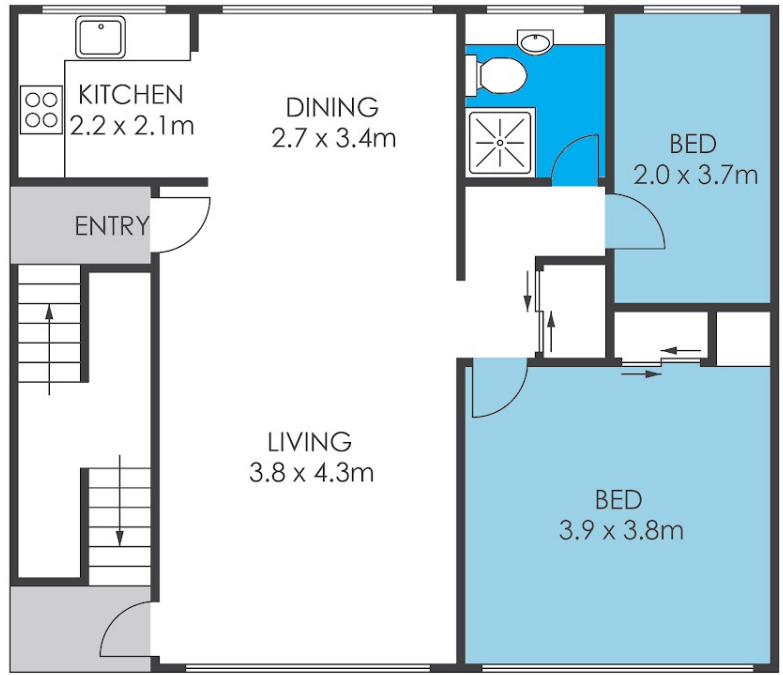
UPPER LEVEL
