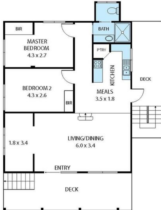
UPPER LEVEL
