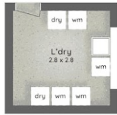
:: FLOOR PLAN Shared Laundry (Not Actual Location)
