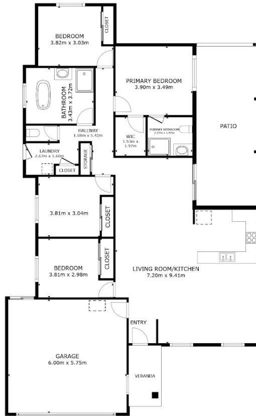
FLOOR PLAN
