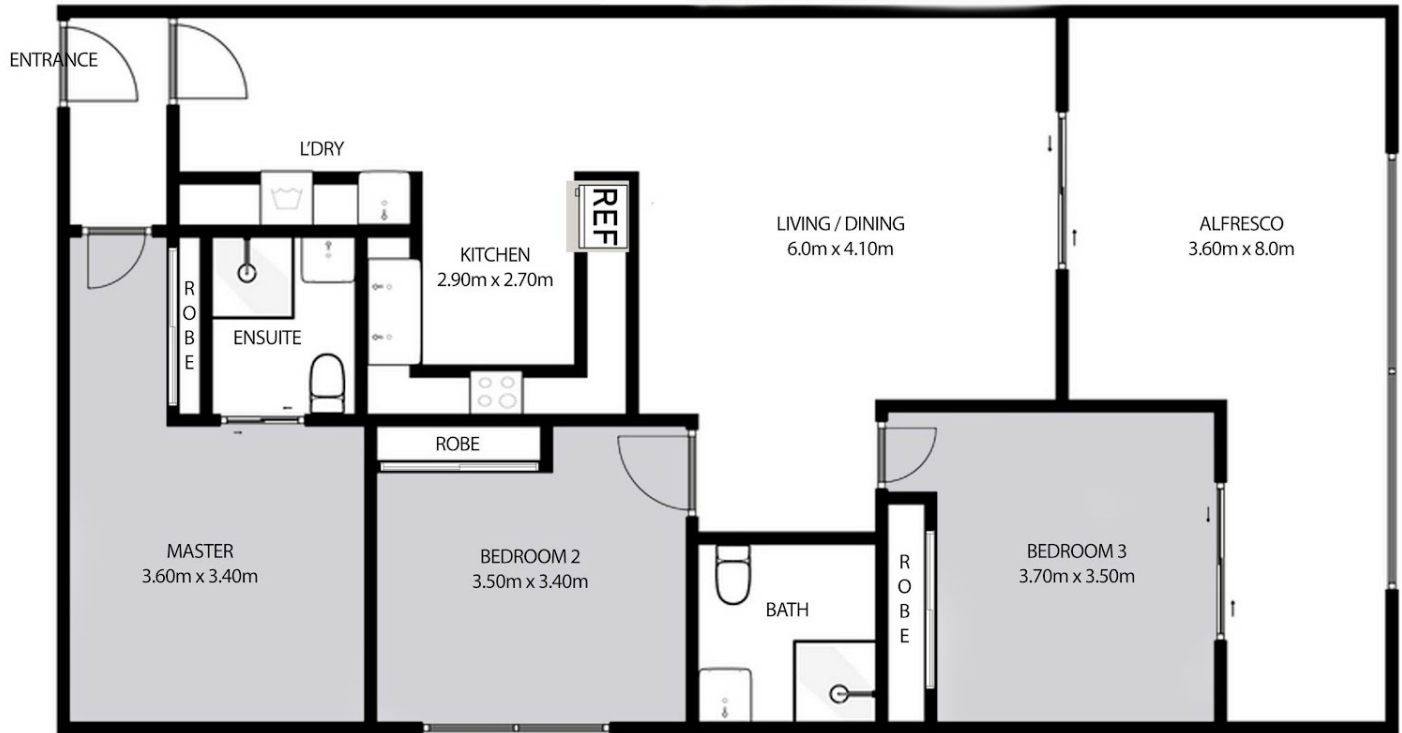
FLOOR PLAN
