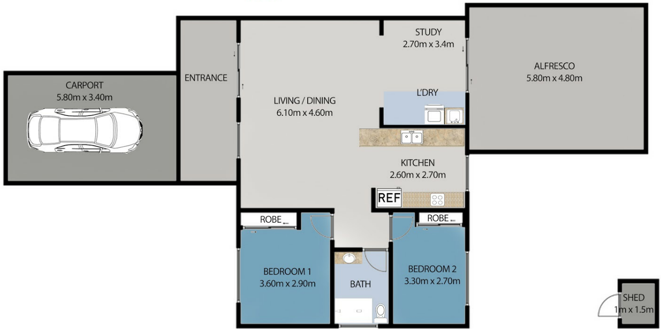
FLOOR PLAN
