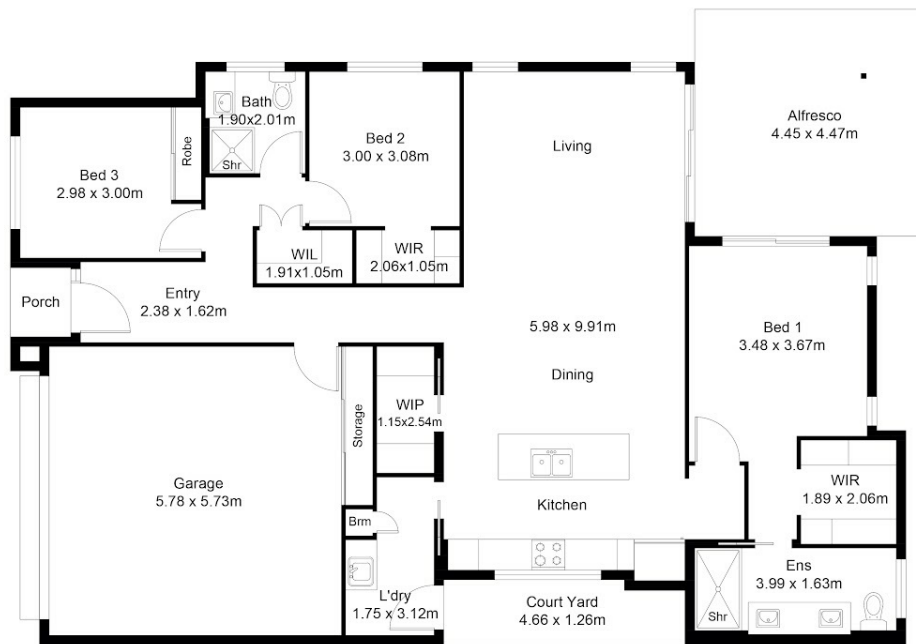
FLOOR PLAN
