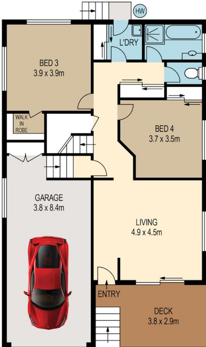
LOWER LEVEL
