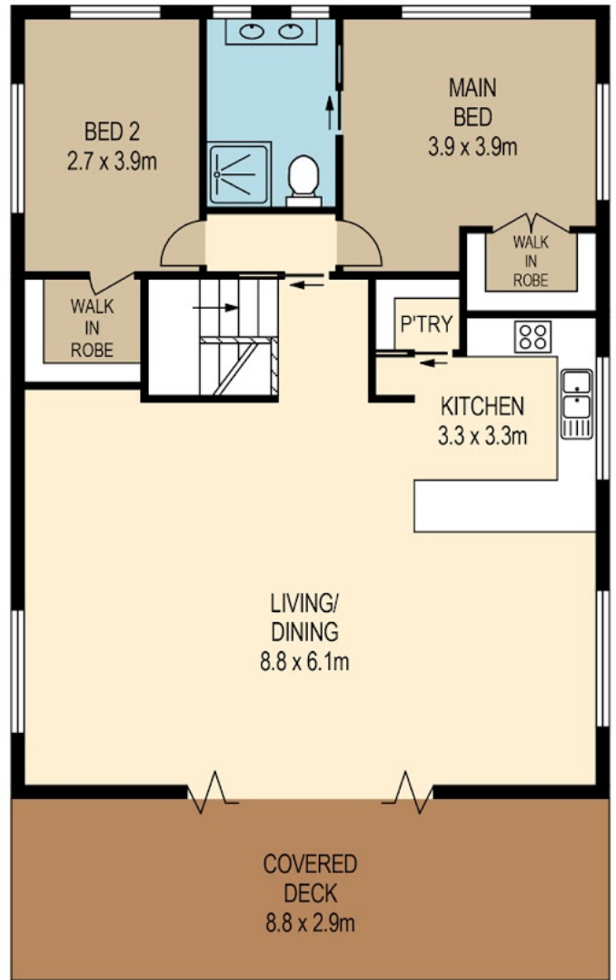
UPPER LEVEL
