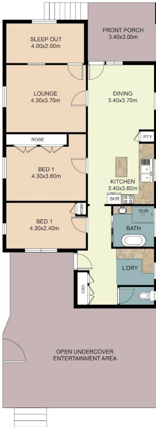
FLOOR PLAN
