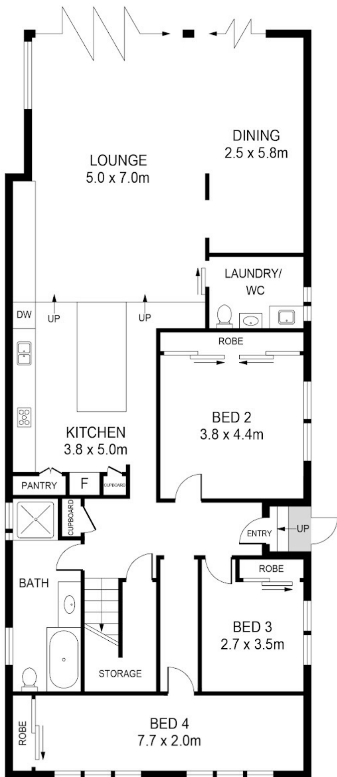
GROUND FLOOR
