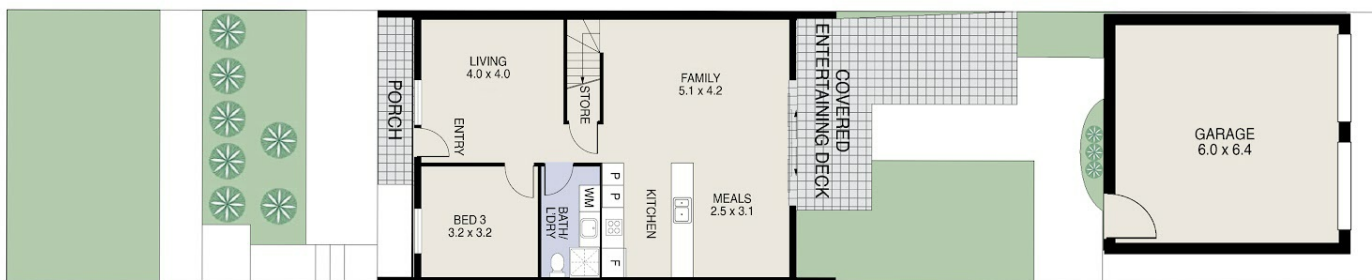
GROUND FLOOR
