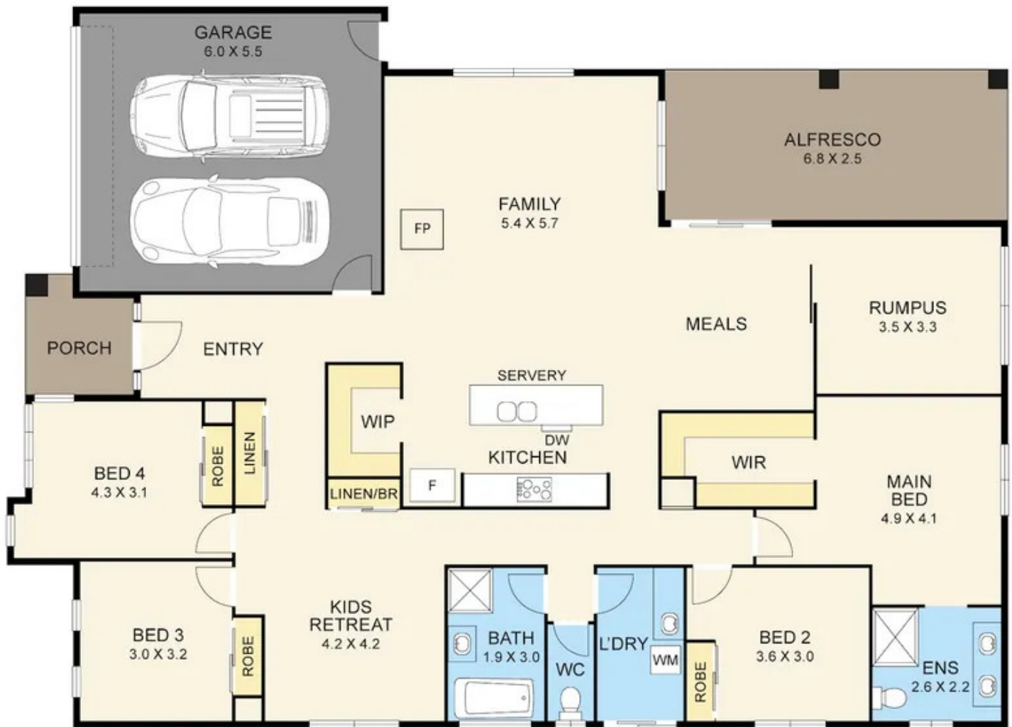
FLOOR PLAN
