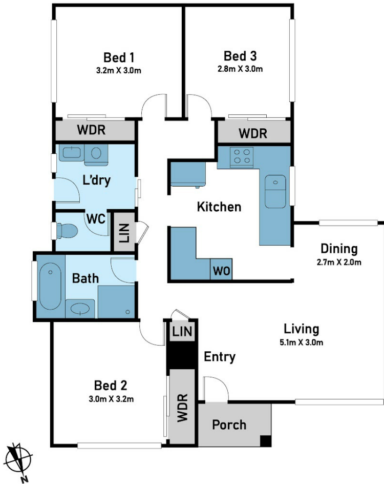
Floor Plan
