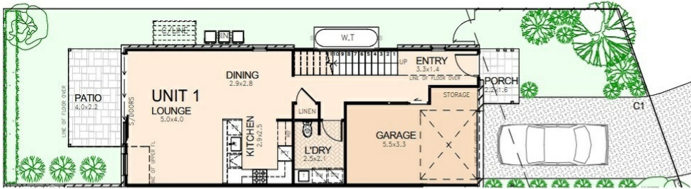
GROUND FLOOR
