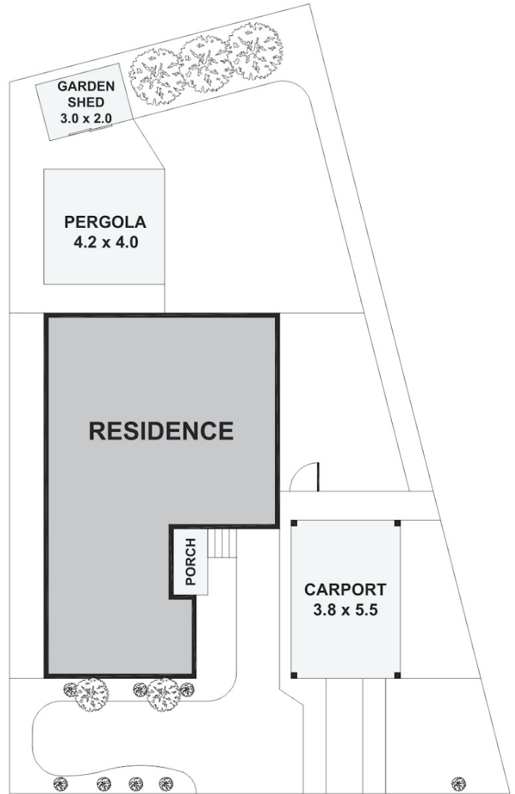
SITE PLAN
