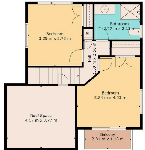
Floor 2
