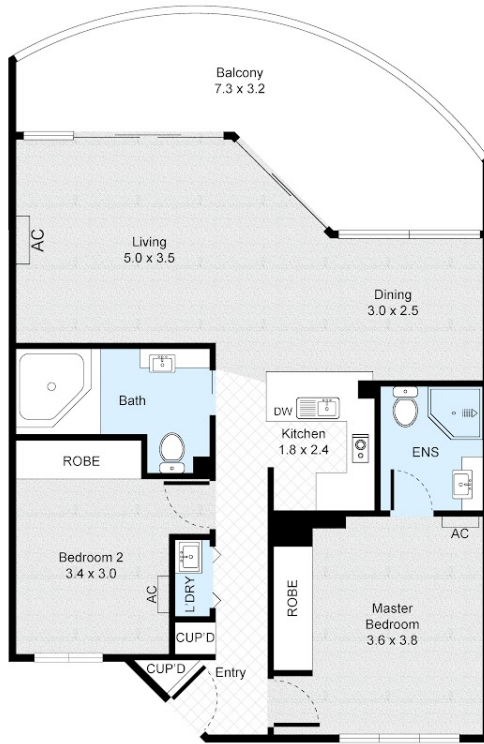
FLOOR PLAN
