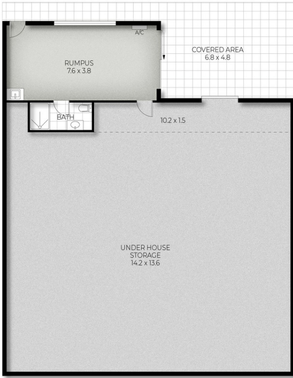
LOWER LEVEL
