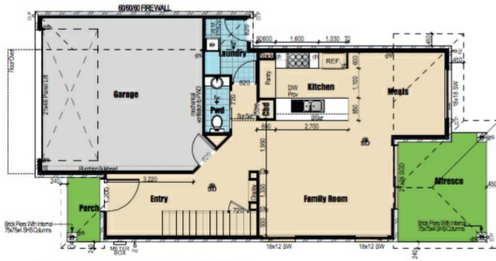
Ground Floor 1:100
