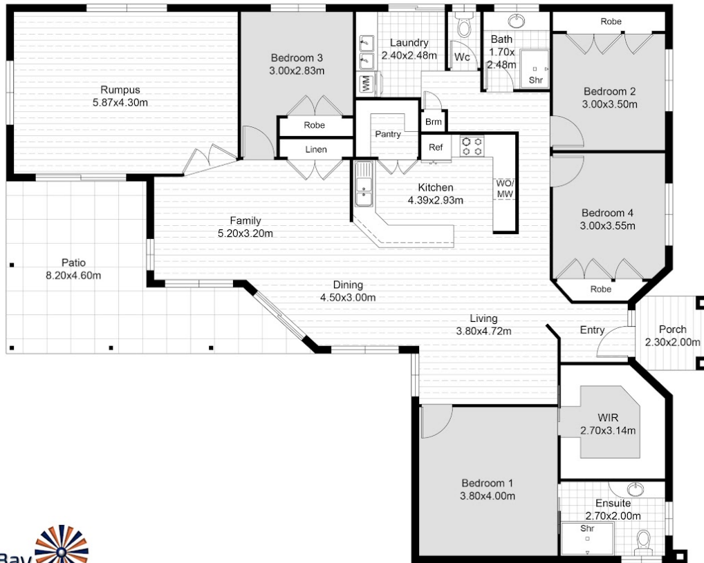
FLOOR PLAN
