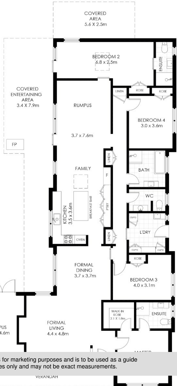
GROUND LEVEL
