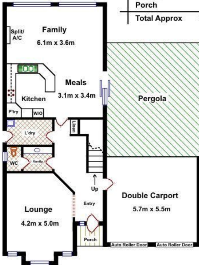
Lower Floor
