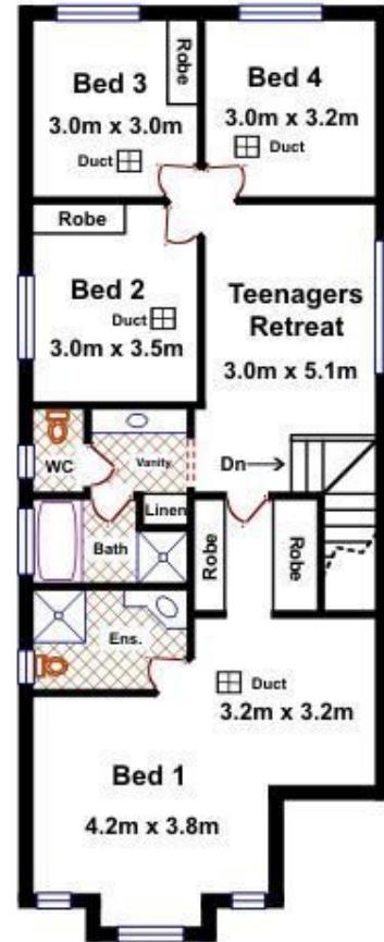
Upper Floor
